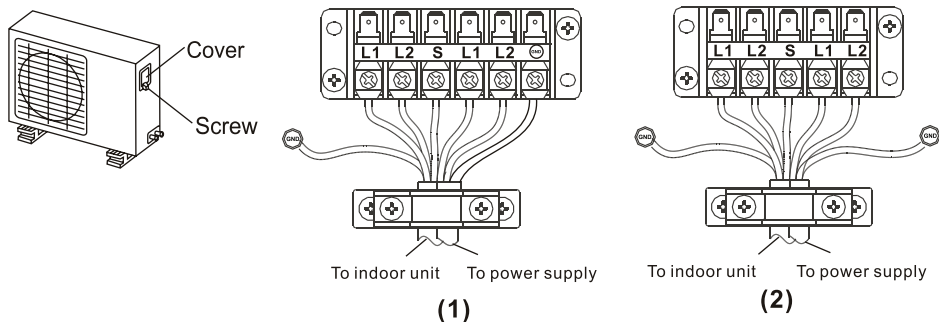
Terminal block of outdoor unit
